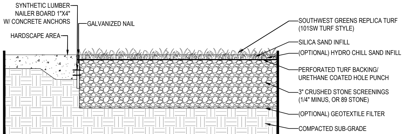
TYPICAL INSTALL CROSS SECTION
