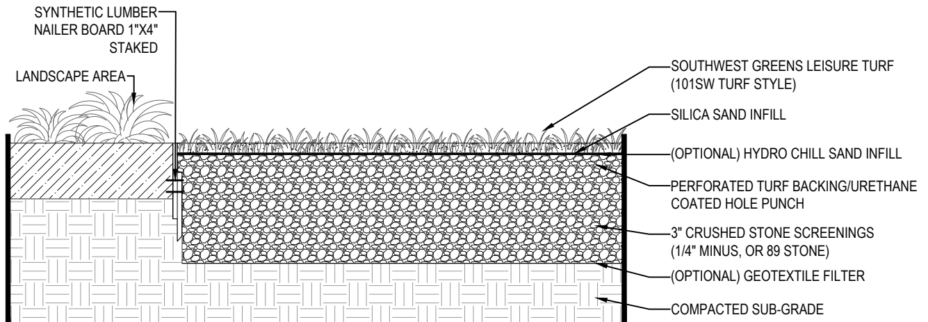
TYPICAL INSTALL CROSS SECTION
