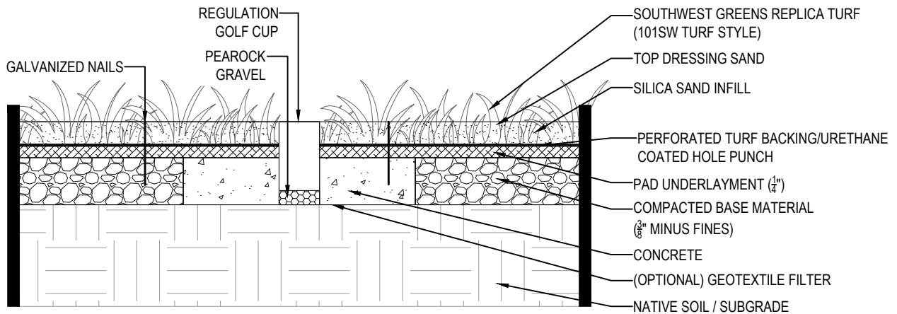
TYPICAL INSTALL CROSS SECTION
