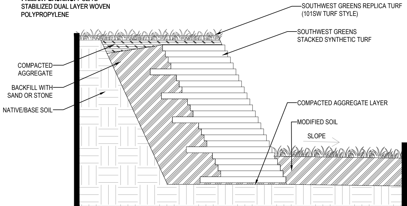
TYPICAL INSTALL CROSS SECTION
