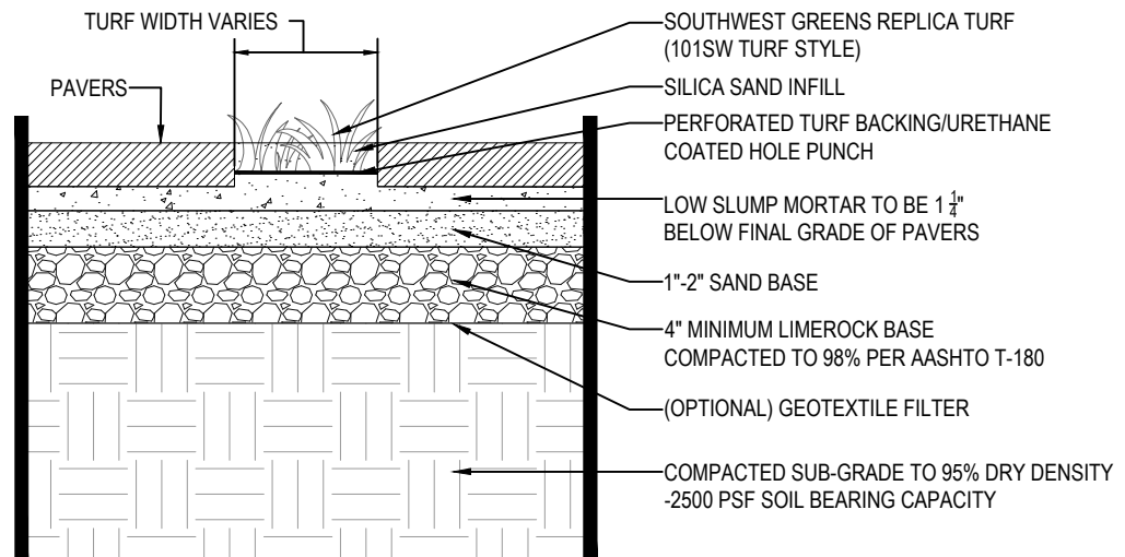
TYPICAL INSTALL CROSS SECTION
