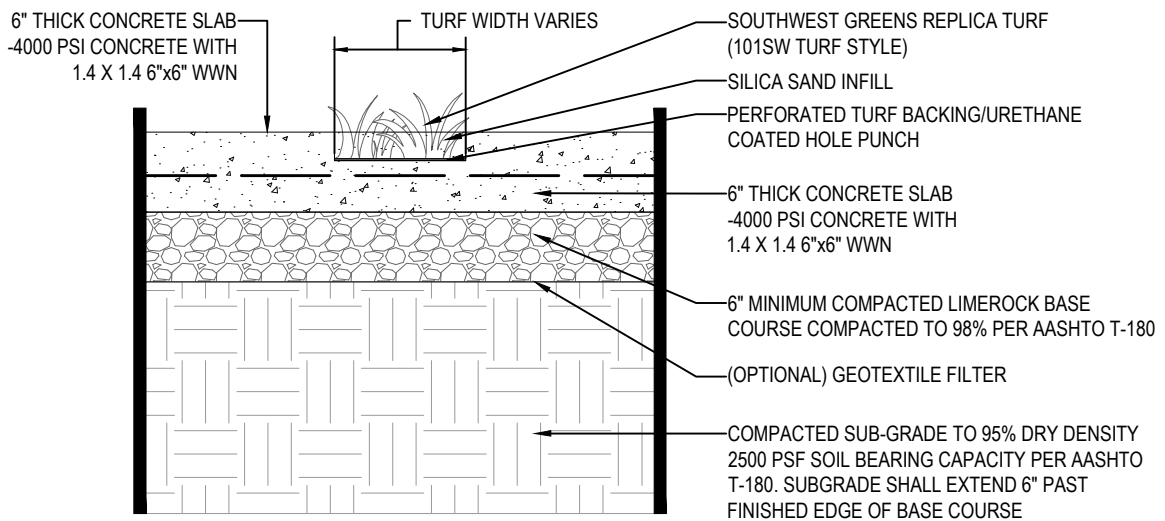
TYPICAL INSTALL CROSS SECTION
