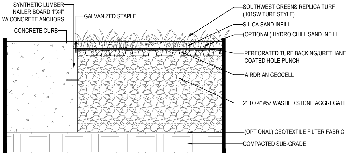
TYPICAL INSTALL CROSS SECTION
