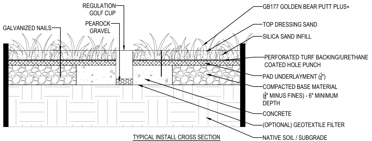
TYPICAL INSTALL CROSS SECTION
